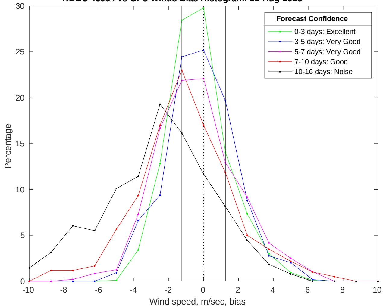
NDBC 46054 vs GFS Winds Bias Histogram: 21-Aug-2025
