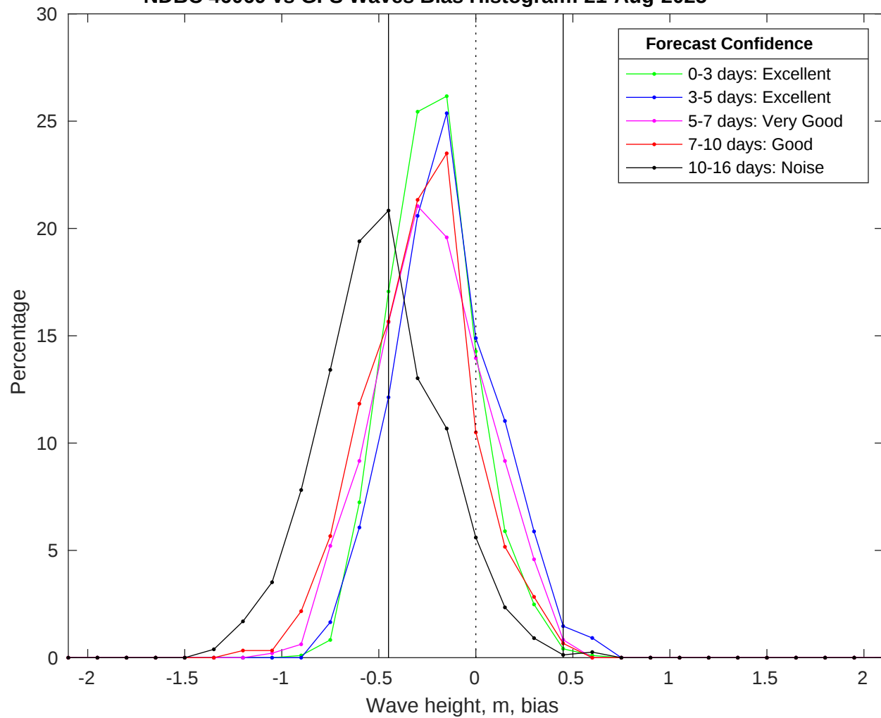
NDBC 46069 vs GFS Waves Bias Histogram: 21-Aug-2025
