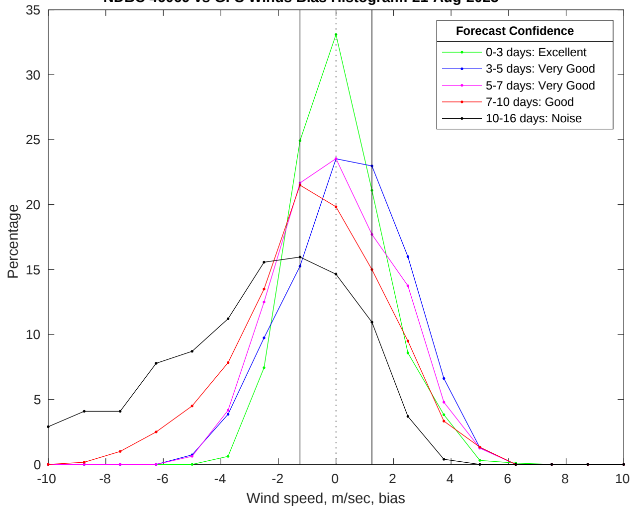
NDBC 46069 vs GFS Winds Bias Histogram: 21-Aug-2025
