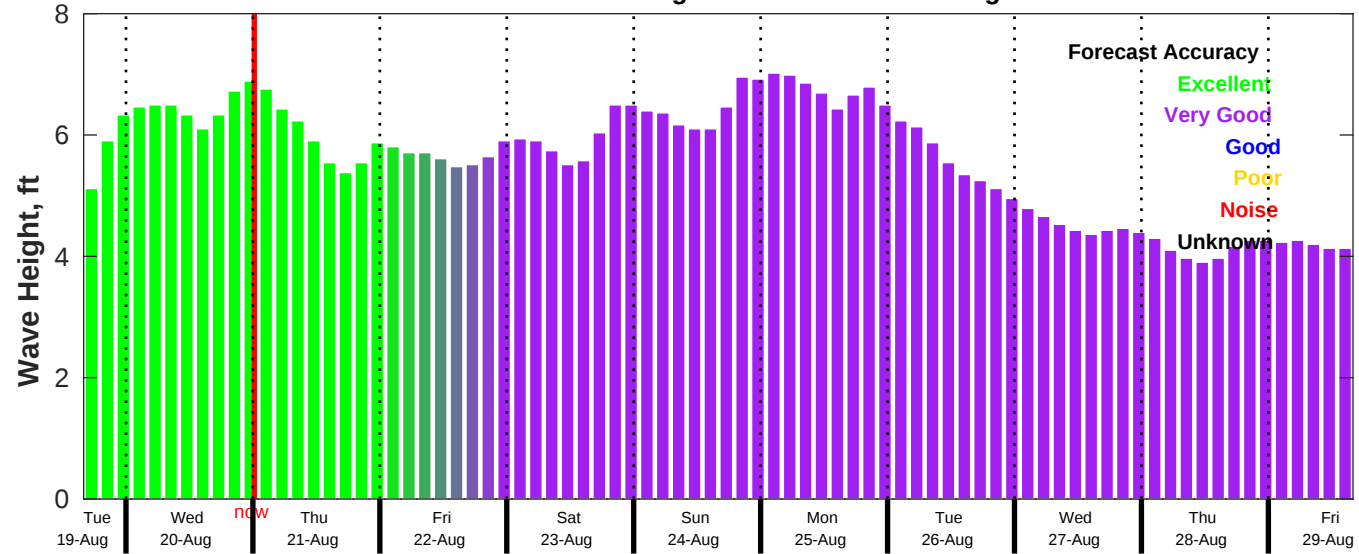
CMEMS Wave Forecast for NDBC 46069 from 19-Aug-2025 16:00:00 to 29-Aug-2025 16:00:00
