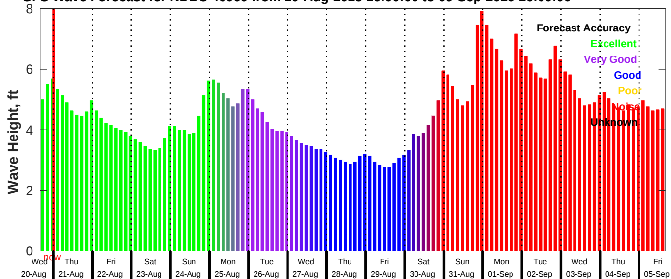
GFS Wave Forecast for NDBC 46069 from 20-Aug-2025 16:00:00 to 05-Sep-2025 16:00:00
