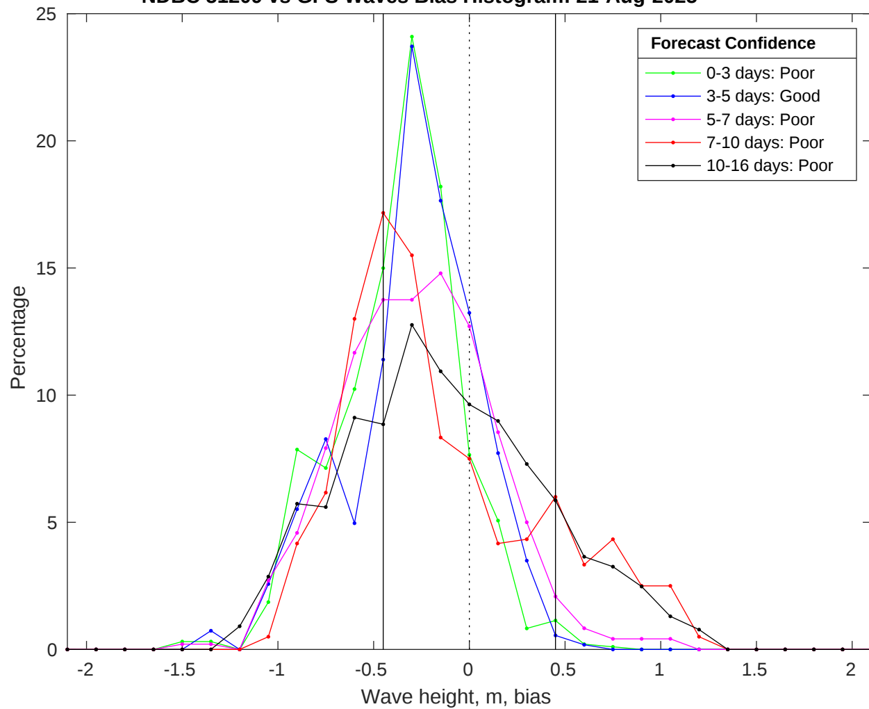
NDBC 51209 vs GFS Waves Bias Histogram: 21-Aug-2025
