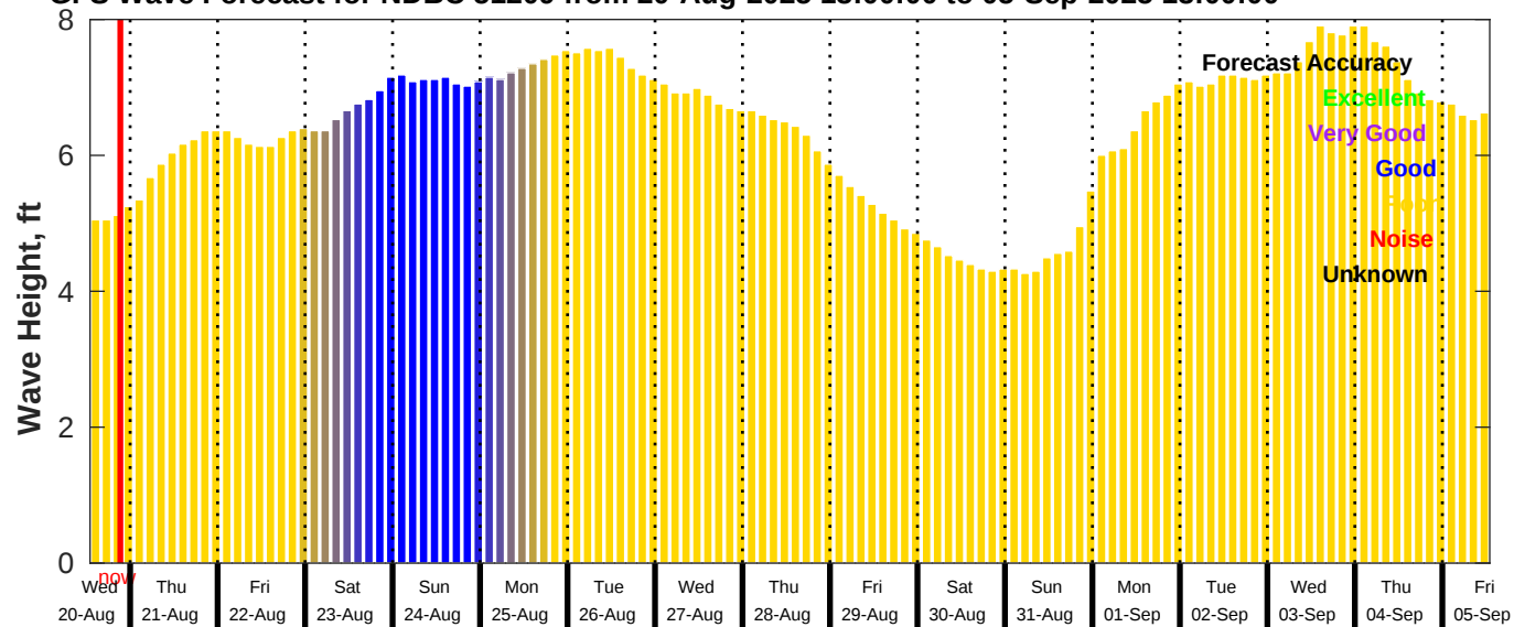
GFS Wave Forecast for NDBC 51209 from 20-Aug-2025 13:00:00 to 05-Sep-2025 13:00:00
