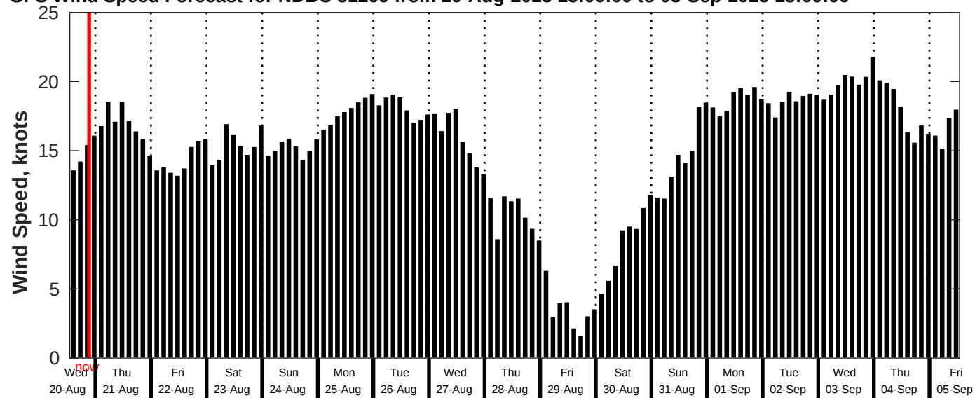
GFS Wind Speed Forecast for NDBC 51209 from 20-Aug-2025 13:00:00 to 05-Sep-2025 13:00:00
