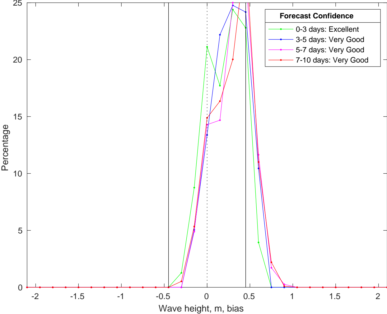
NDBC 51211 vs CMEMS Waves Bias Histogram: 21-Aug-2025
