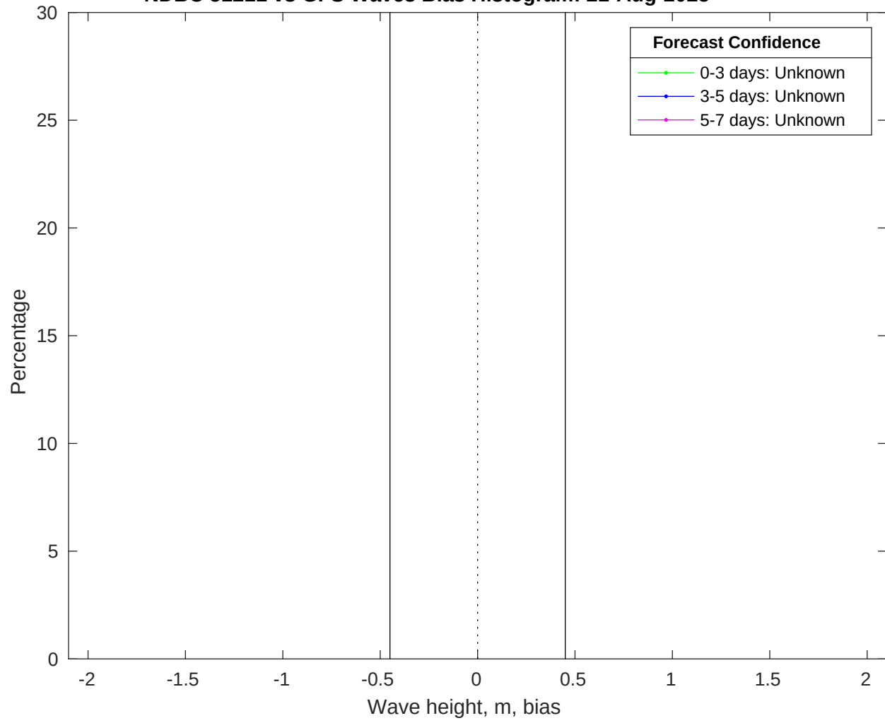
NDBC 51211 vs GFS Waves Bias Histogram: 21-Aug-2025
