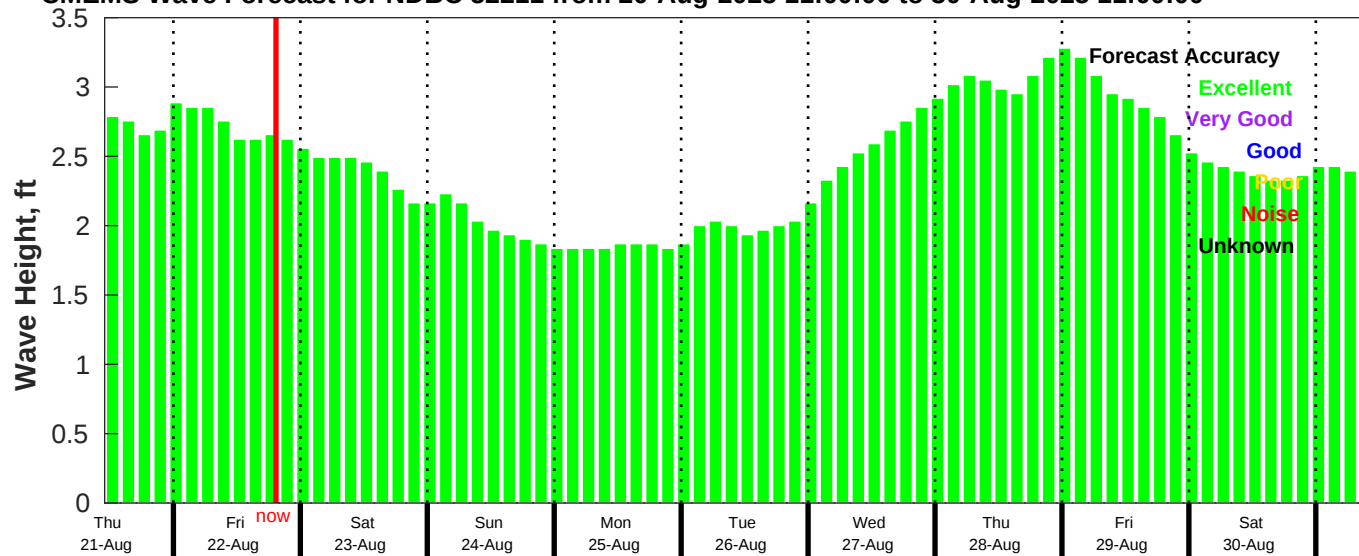
CMEMS Wave Forecast for NDBC 52211 from 20-Aug-2025 11:00:00 to 30-Aug-2025 11:00:00
