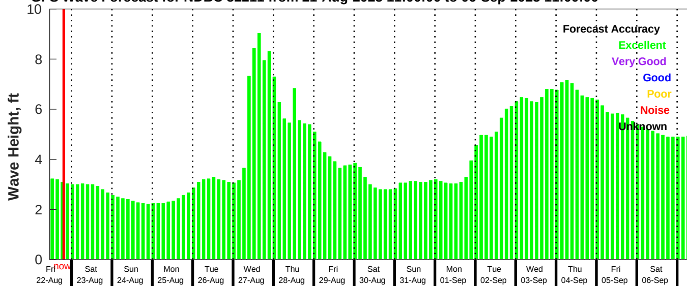
GFS Wave Forecast for NDBC 52211 from 21-Aug-2025 11:00:00 to 06-Sep-2025 11:00:00
