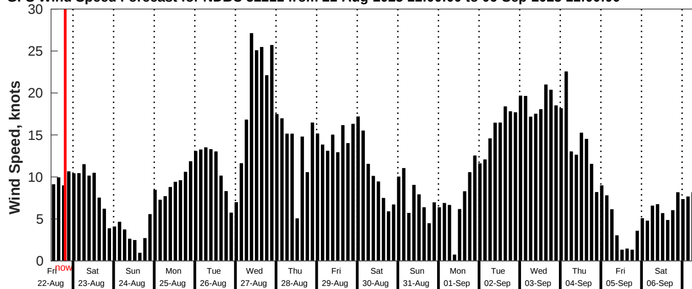
GFS Wind Speed Forecast for NDBC 52211 from 21-Aug-2025 11:00:00 to 06-Sep-2025 11:00:00
