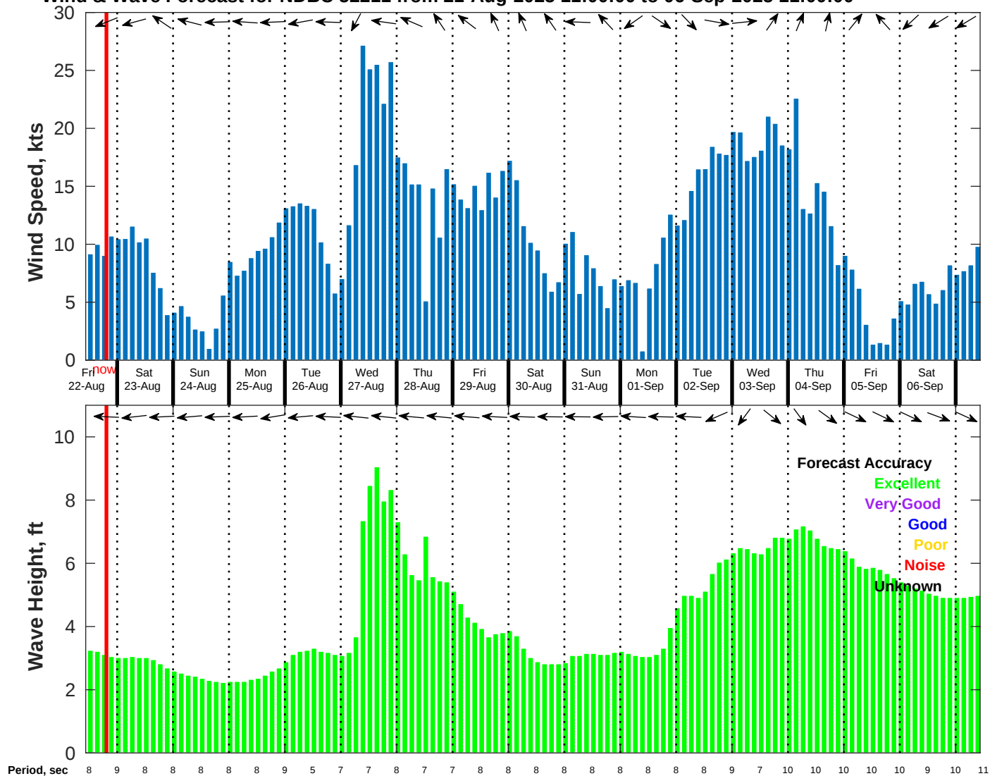
Wind & Wave Forecast for NDBC 52211 from 21-Aug-2025 11:00:00 to 06-Sep-2025 11:00:00
