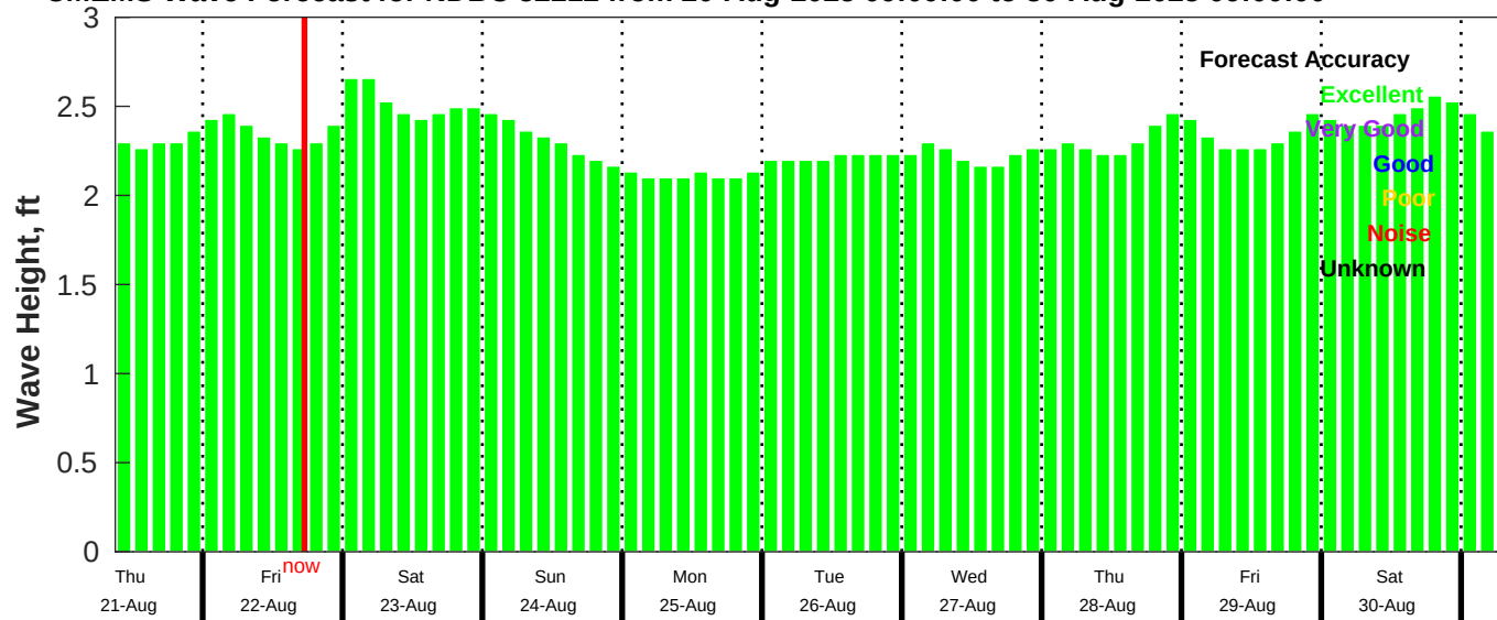
CMEMS Wave Forecast for NDBC 52212 from 20-Aug-2025 09:00:00 to 30-Aug-2025 09:00:00
