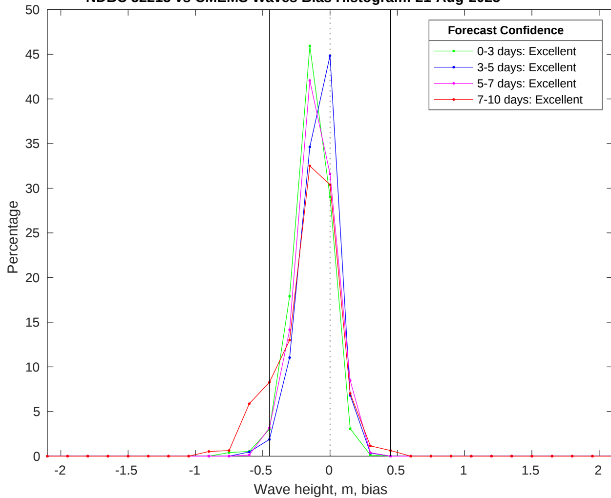
NDBC 52213 vs CMEMS Waves Bias Histogram: 21-Aug-2025
