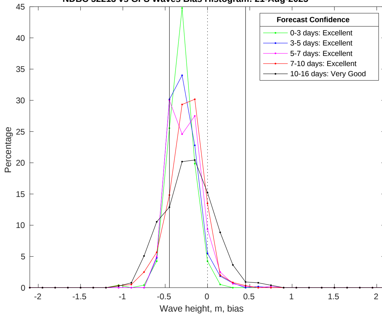
NDBC 52213 vs GFS Waves Bias Histogram: 21-Aug-2025
