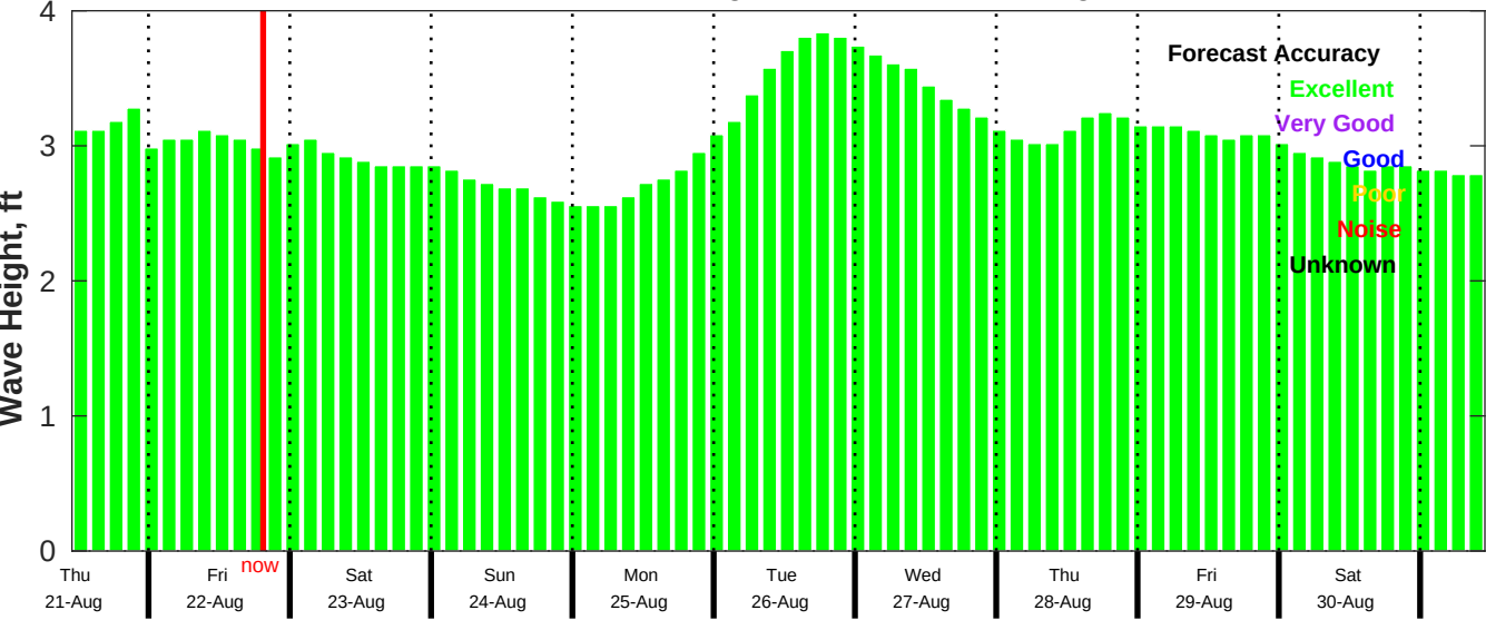
CMEMS Wave Forecast for NDBC 52213 from 20-Aug-2025 11:00:00 to 30-Aug-2025 11:00:00
