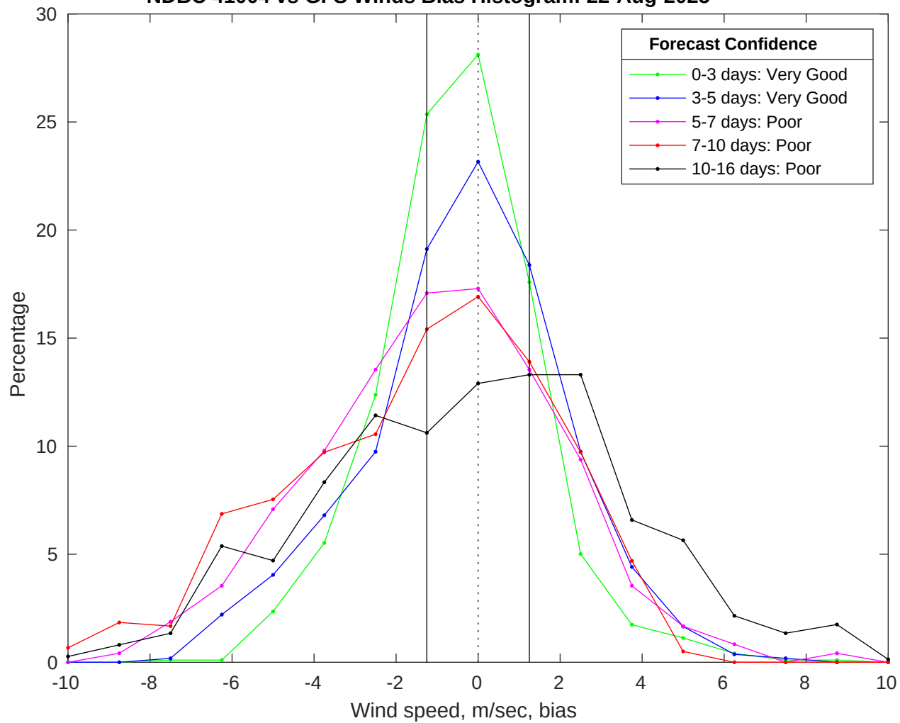
NDBC 41004 vs GFS Winds Bias Histogram: 22-Aug-2025
