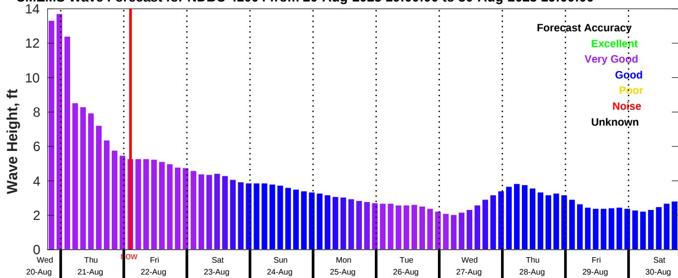
CMEMS Wave Forecast for NDBC 41004 from 20-Aug-2025 19:00:00 to 30-Aug-2025 19:00:00
