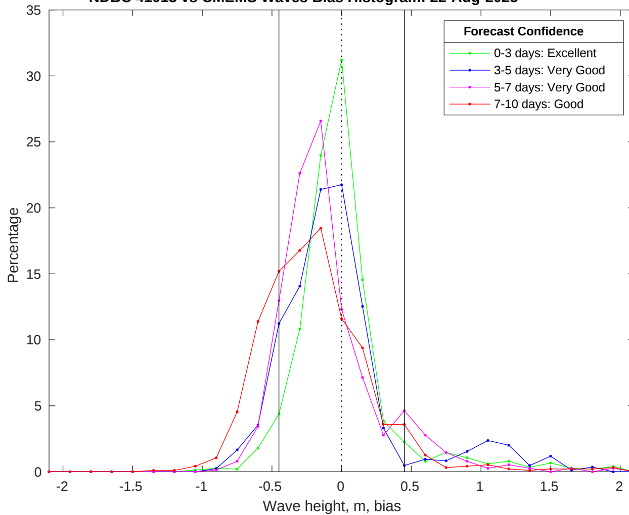
NDBC 41013 vs CMEMS Waves Bias Histogram: 22-Aug-2025
