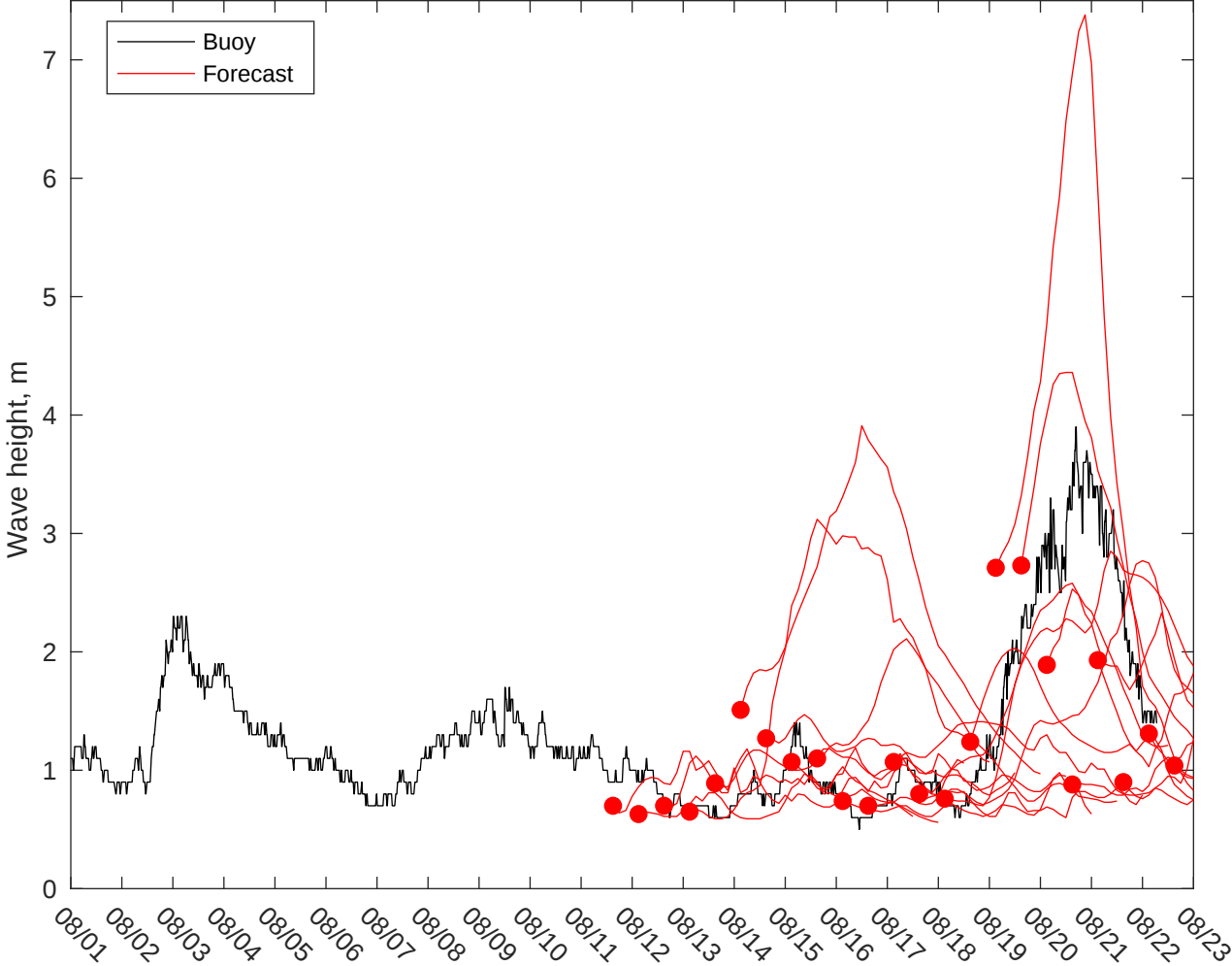
NDBC 41013 vs GFS Waves: 10 to 16 day forecast
