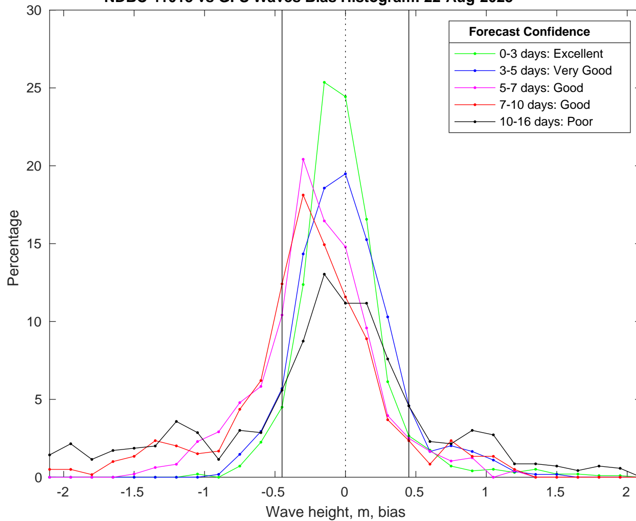
NDBC 41013 vs GFS Waves Bias Histogram: 22-Aug-2025
