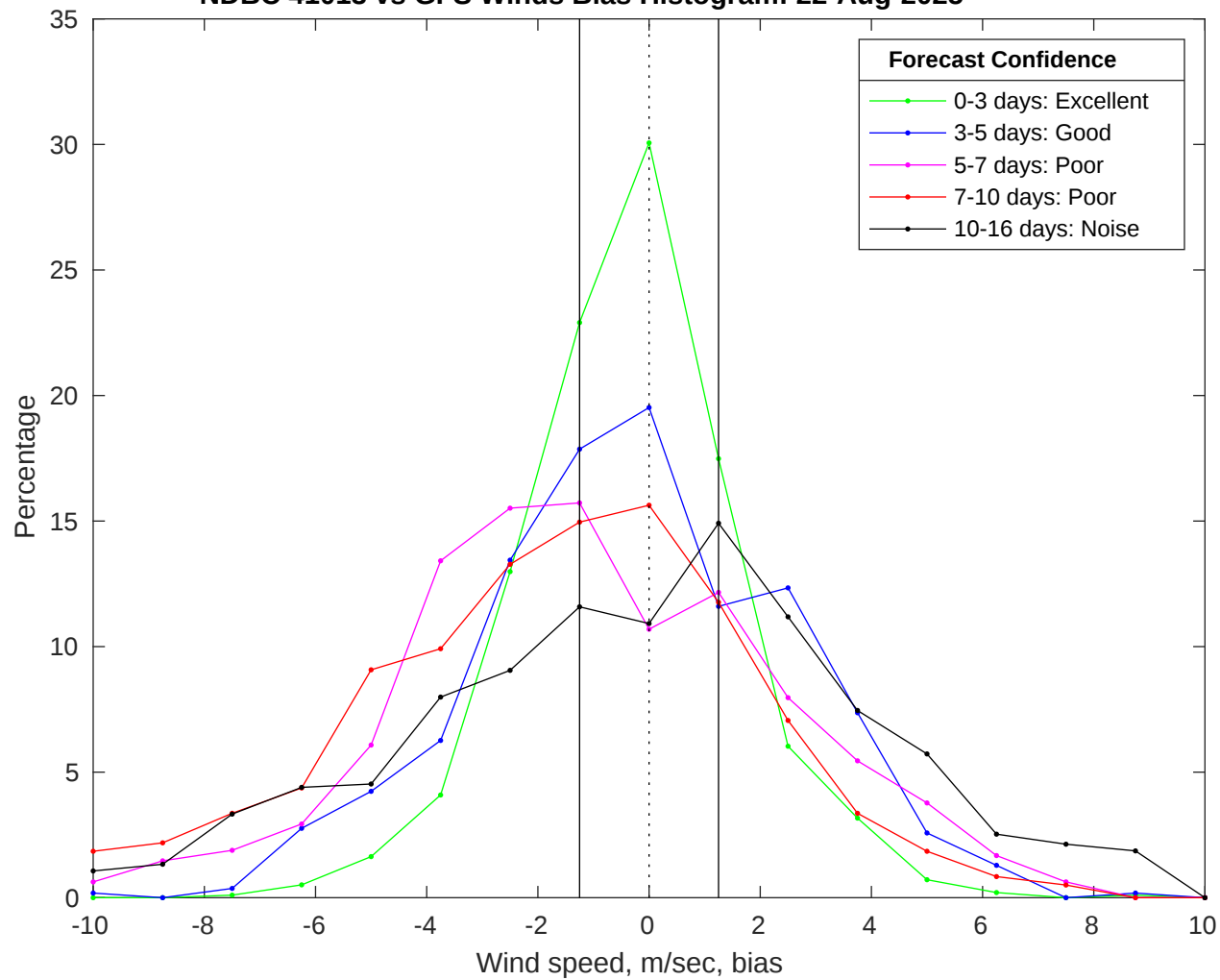
NDBC 41013 vs GFS Winds Bias Histogram: 22-Aug-2025
