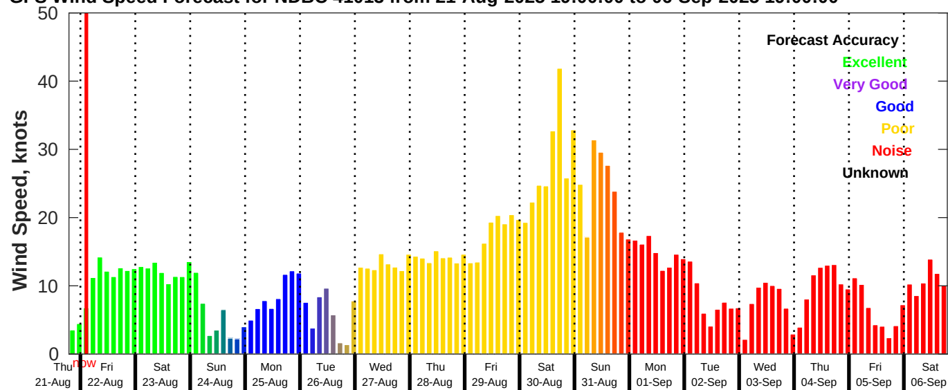
GFS Wind Speed Forecast for NDBC 41013 from 21-Aug-2025 19:00:00 to 06-Sep-2025 19:00:00
