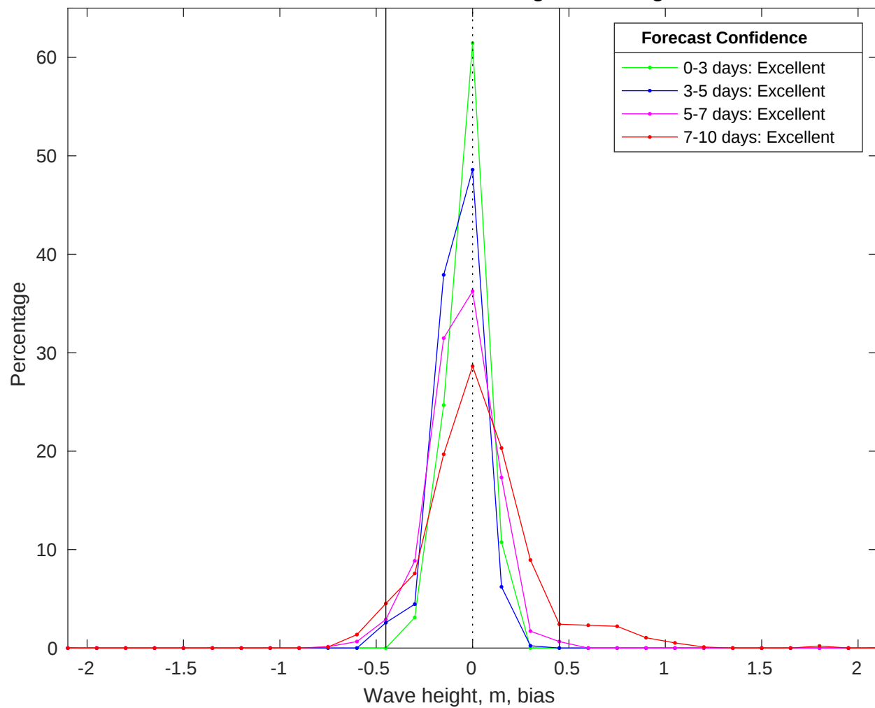
NDBC 41040 vs CMEMS Waves Bias Histogram: 22-Aug-2025
