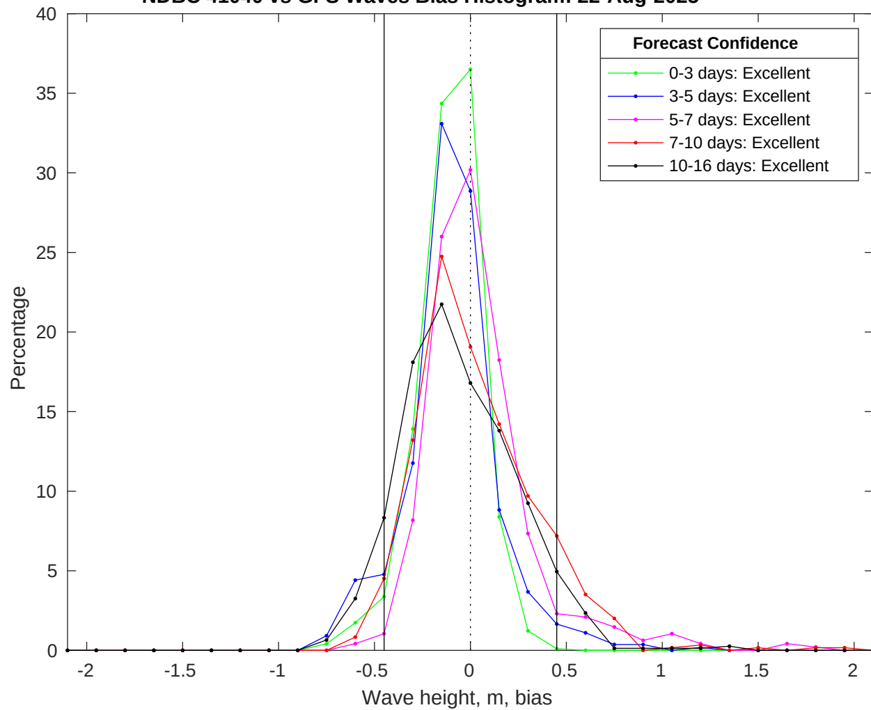
NDBC 41040 vs GFS Waves Bias Histogram: 22-Aug-2025
