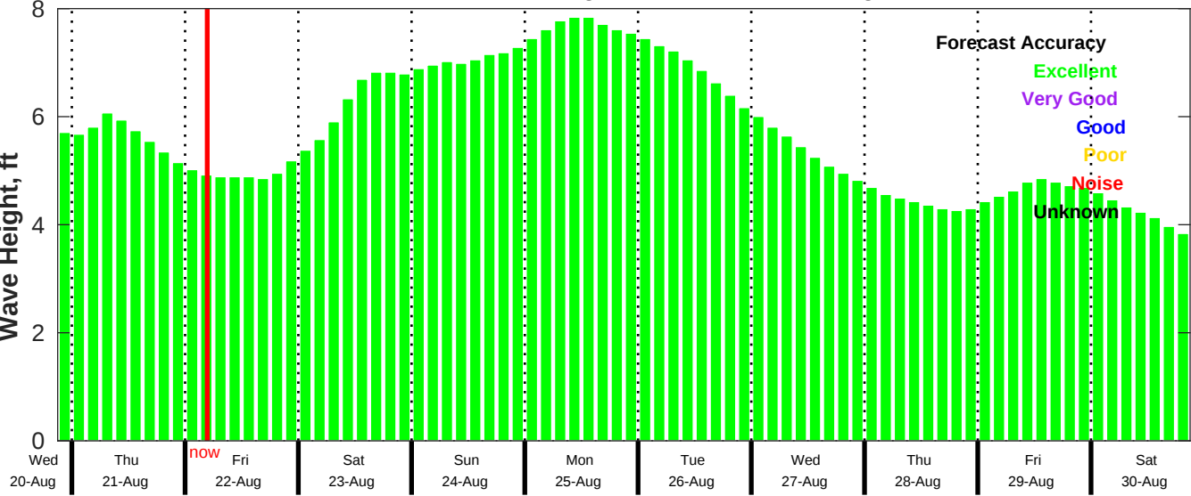
CMEMS Wave Forecast for NDBC 41040 from 20-Aug-2025 21:00:00 to 30-Aug-2025 21:00:00
