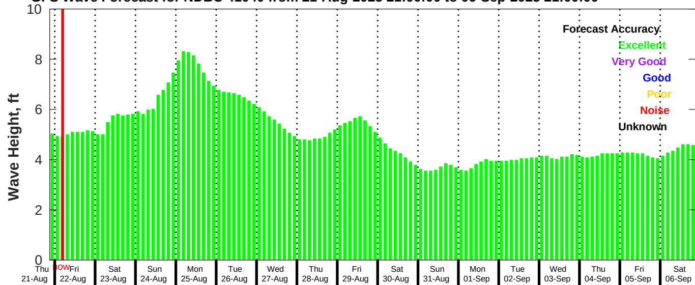
GFS Wave Forecast for NDBC 41040 from 21-Aug-2025 21:00:00 to 06-Sep-2025 21:00:00
