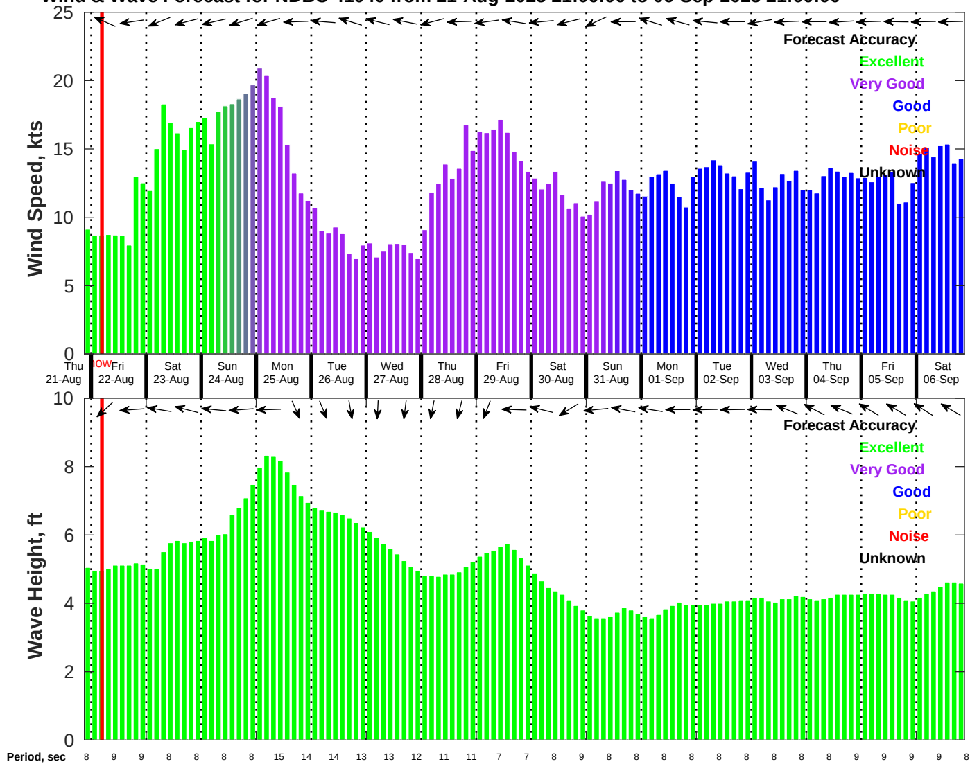
Wind & Wave Forecast for NDBC 41040 from 21-Aug-2025 21:00:00 to 06-Sep-2025 21:00:00
