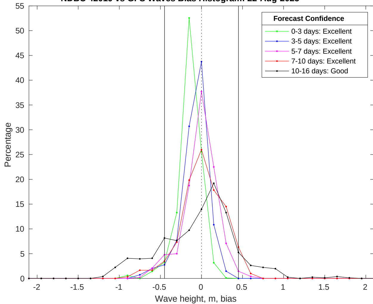
NDBC 42019 vs GFS Waves Bias Histogram: 22-Aug-2025
