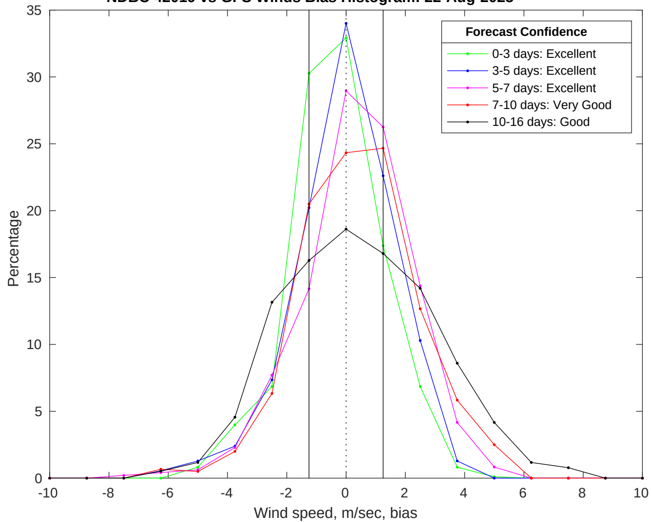
NDBC 42019 vs GFS Winds Bias Histogram: 22-Aug-2025
