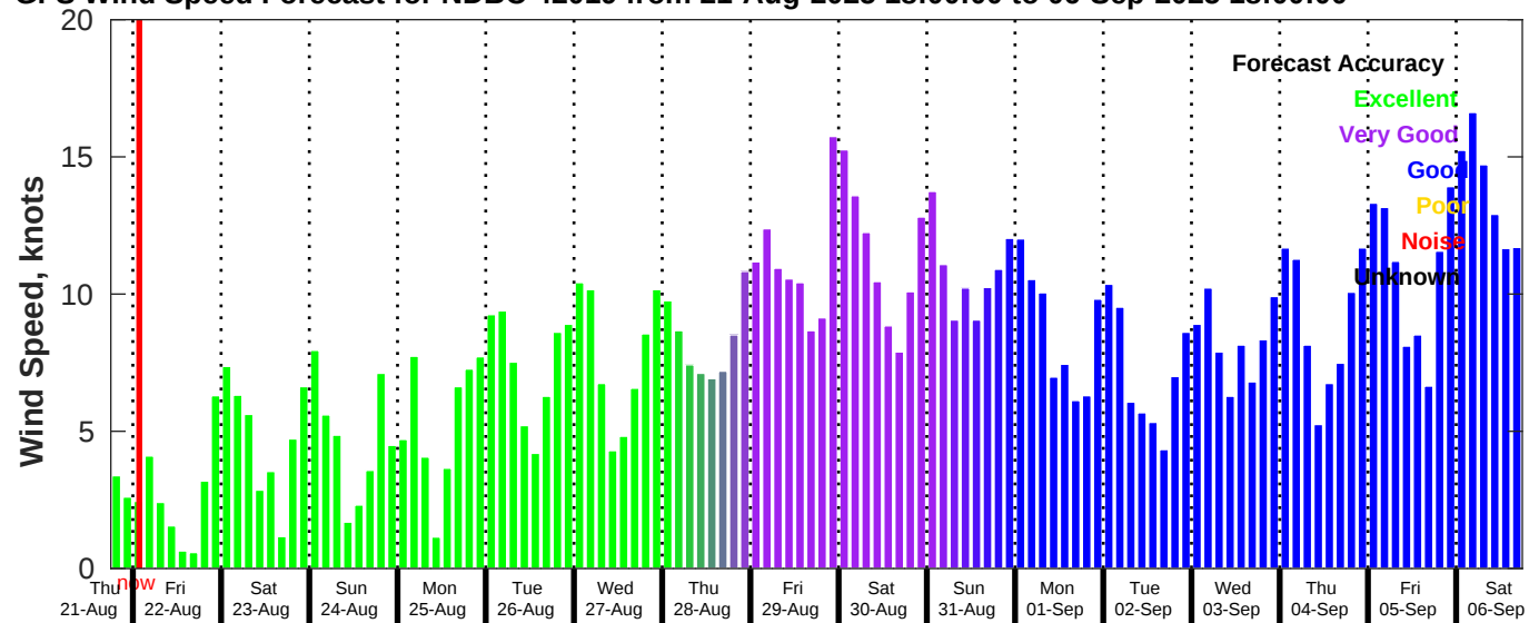
GFS Wind Speed Forecast for NDBC 42019 from 21-Aug-2025 18:00:00 to 06-Sep-2025 18:00:00
