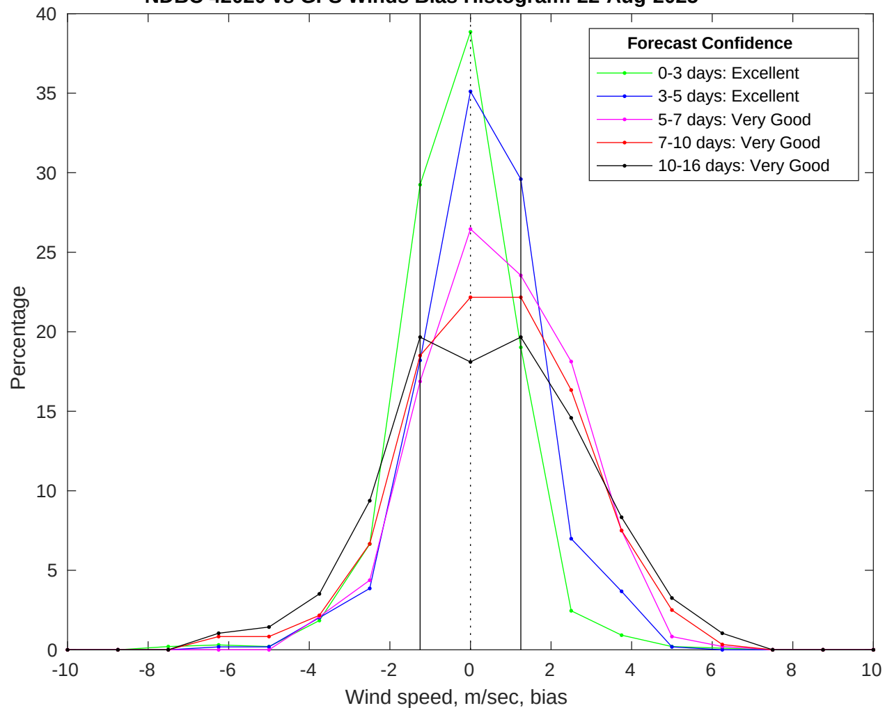
NDBC 42020 vs GFS Winds Bias Histogram: 22-Aug-2025
