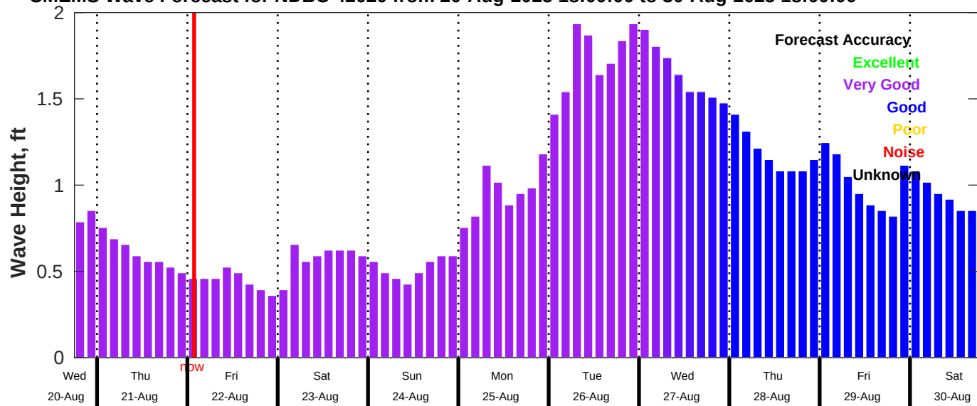
CMEMS Wave Forecast for NDBC 42020 from 20-Aug-2025 18:00:00 to 30-Aug-2025 18:00:00
