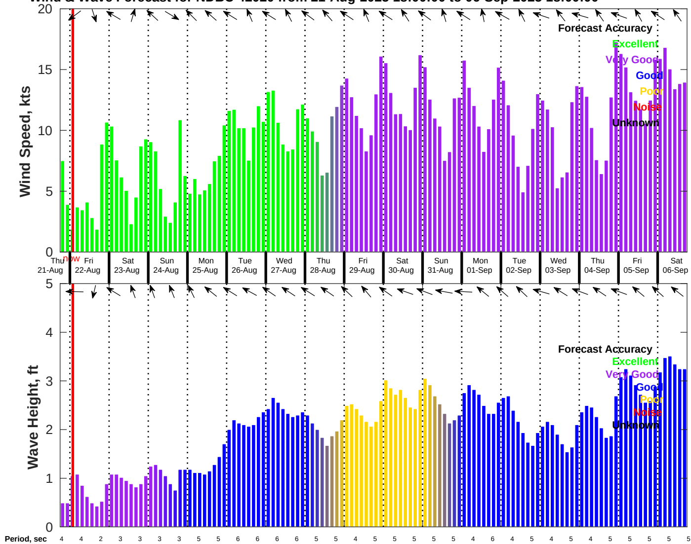
Wind & Wave Forecast for NDBC 42020 from 21-Aug-2025 18:00:00 to 06-Sep-2025 18:00:00
