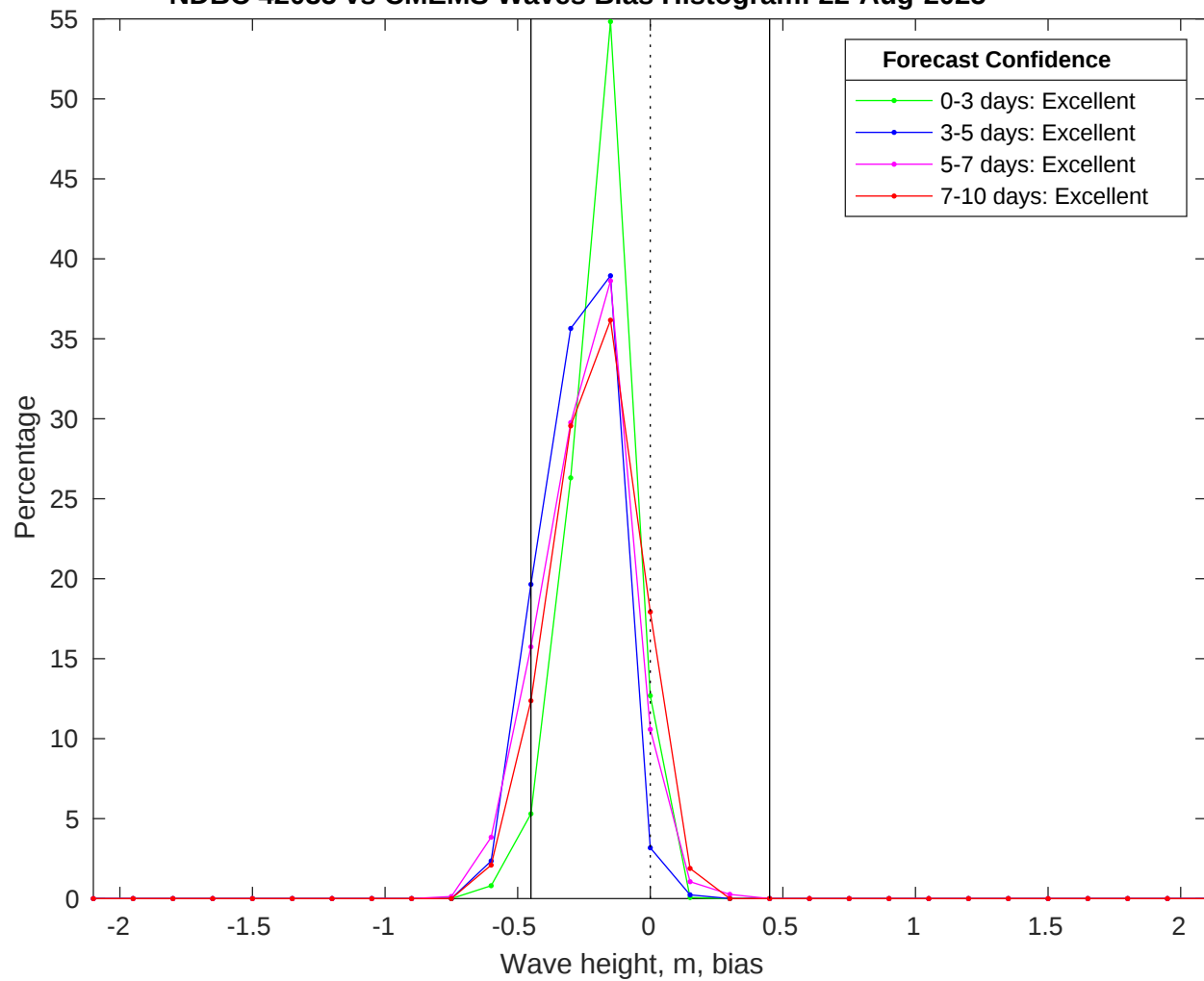
NDBC 42035 vs CMEMS Waves Bias Histogram: 22-Aug-2025
