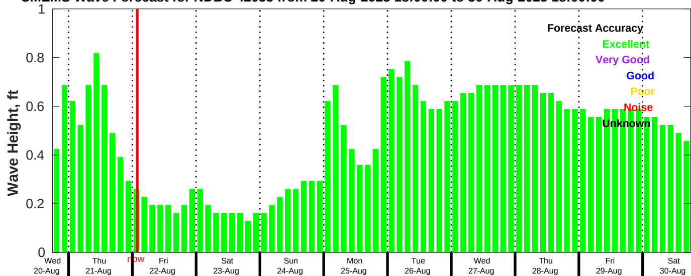
CMEMS Wave Forecast for NDBC 42035 from 20-Aug-2025 18:00:00 to 30-Aug-2025 18:00:00
