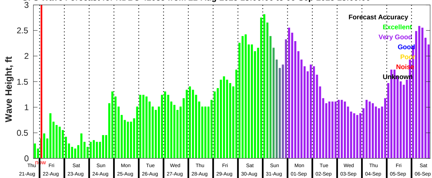
GFS Wave Forecast for NDBC 42035 from 21-Aug-2025 18:00:00 to 06-Sep-2025 18:00:00
