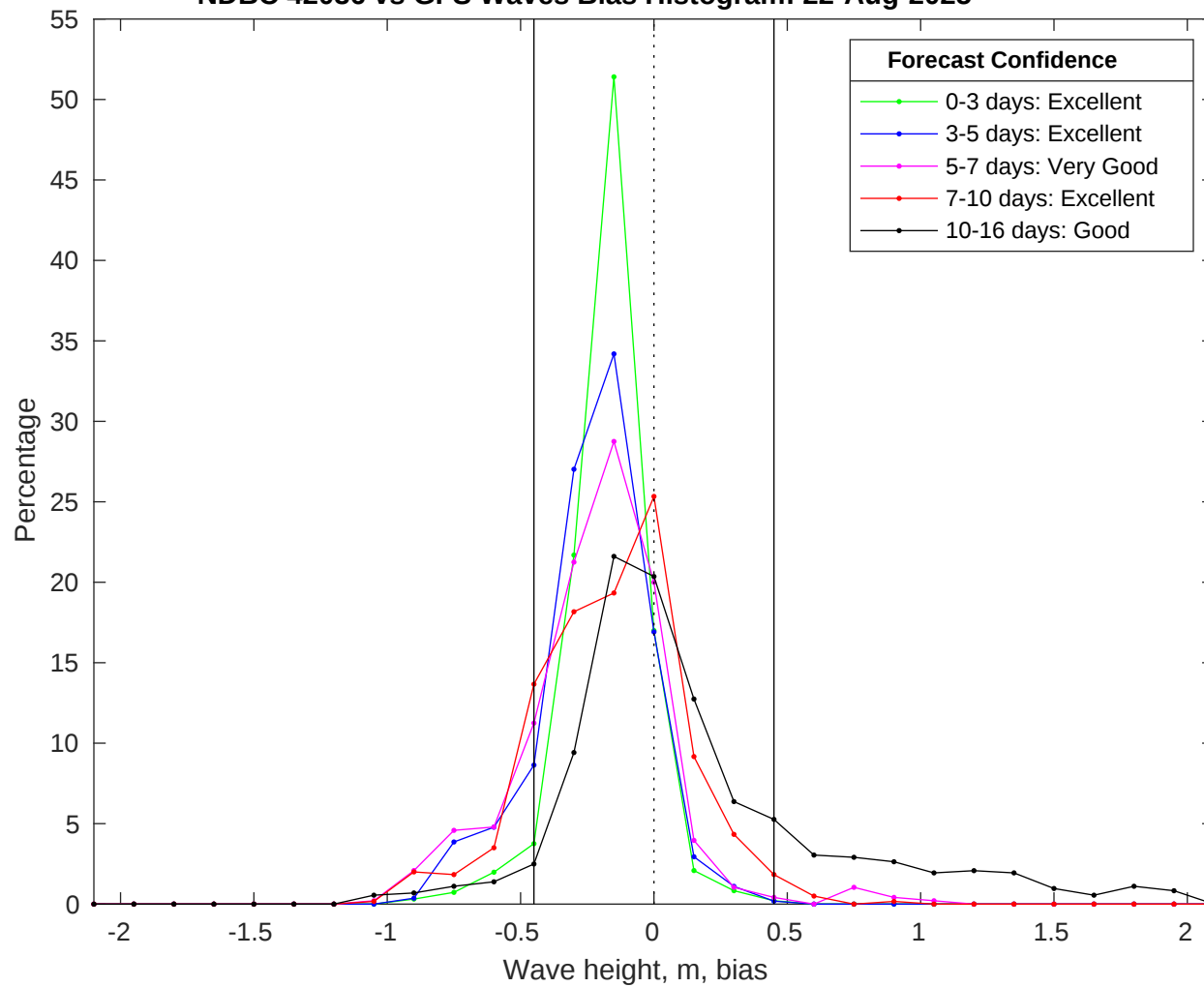
NDBC 42036 vs GFS Waves Bias Histogram: 22-Aug-2025
