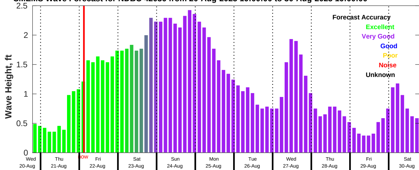
CMEMS Wave Forecast for NDBC 42036 from 20-Aug-2025 19:00:00 to 30-Aug-2025 19:00:00
