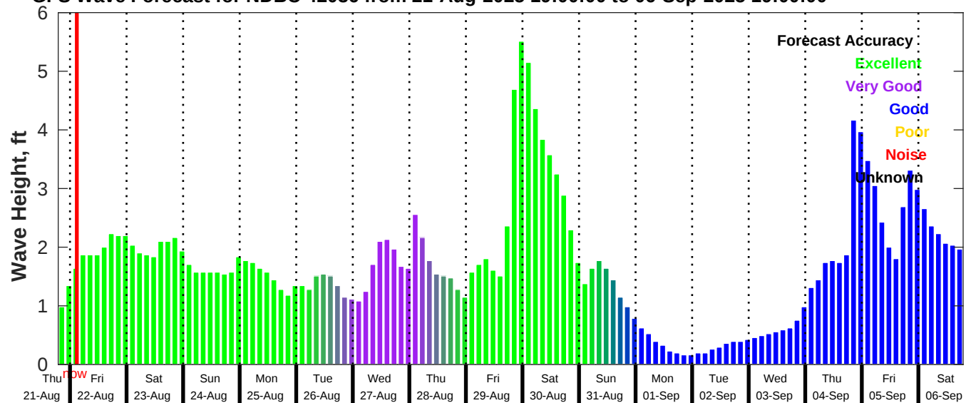
GFS Wave Forecast for NDBC 42036 from 21-Aug-2025 19:00:00 to 06-Sep-2025 19:00:00
