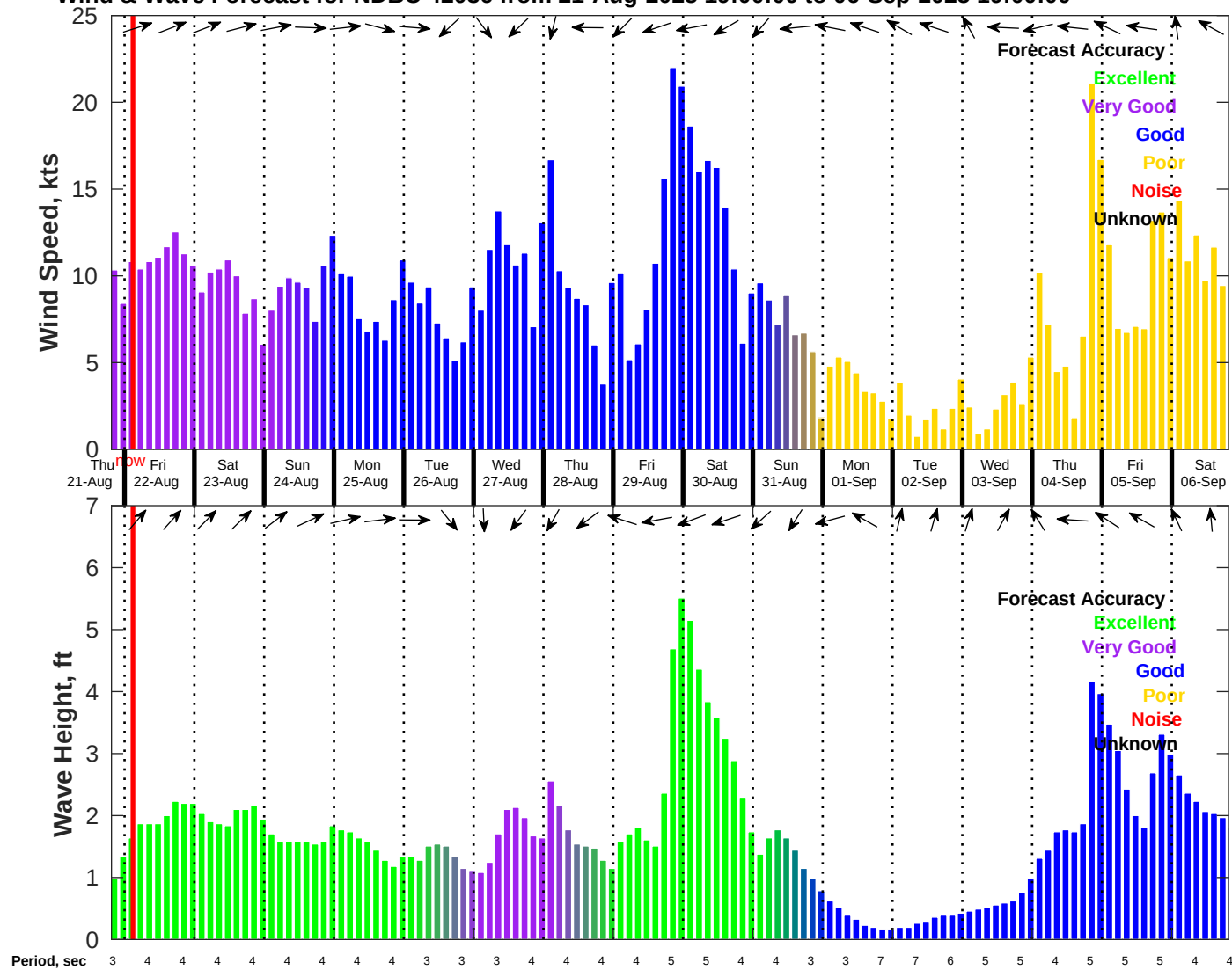
Wind & Wave Forecast for NDBC 42036 from 21-Aug-2025 19:00:00 to 06-Sep-2025 19:00:00
