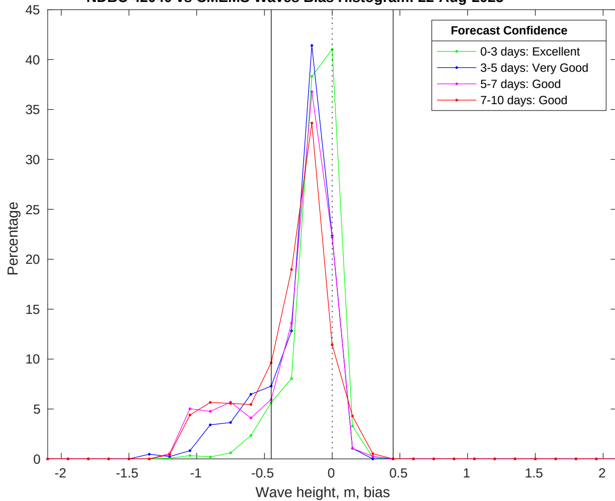
NDBC 42040 vs CMEMS Waves Bias Histogram: 22-Aug-2025
