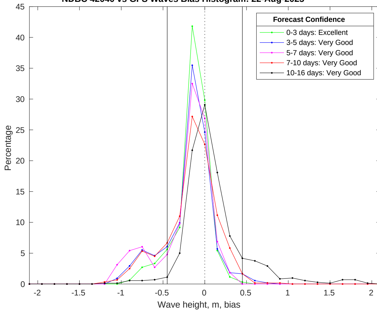
NDBC 42040 vs GFS Waves Bias Histogram: 22-Aug-2025
