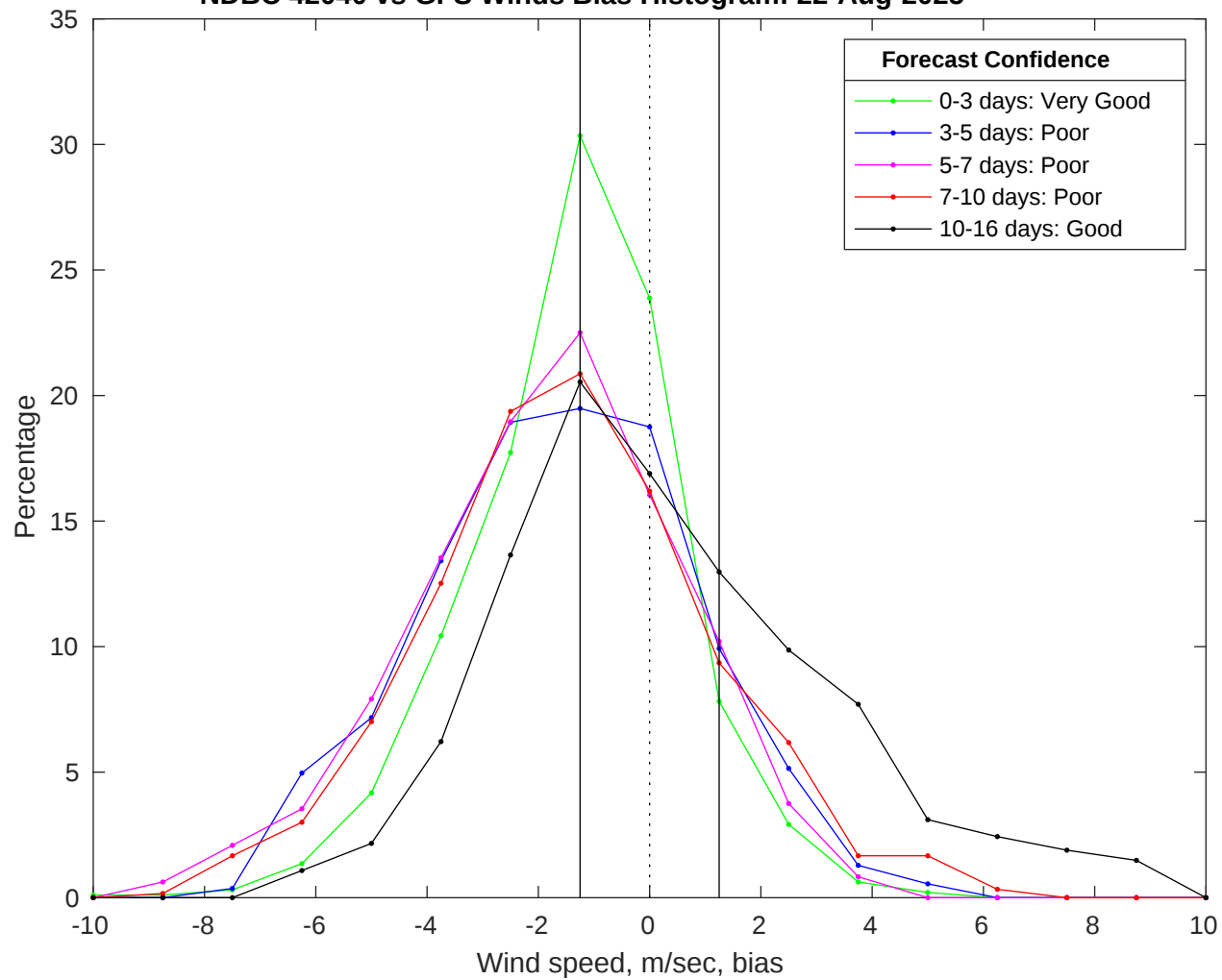
NDBC 42040 vs GFS Winds Bias Histogram: 22-Aug-2025
