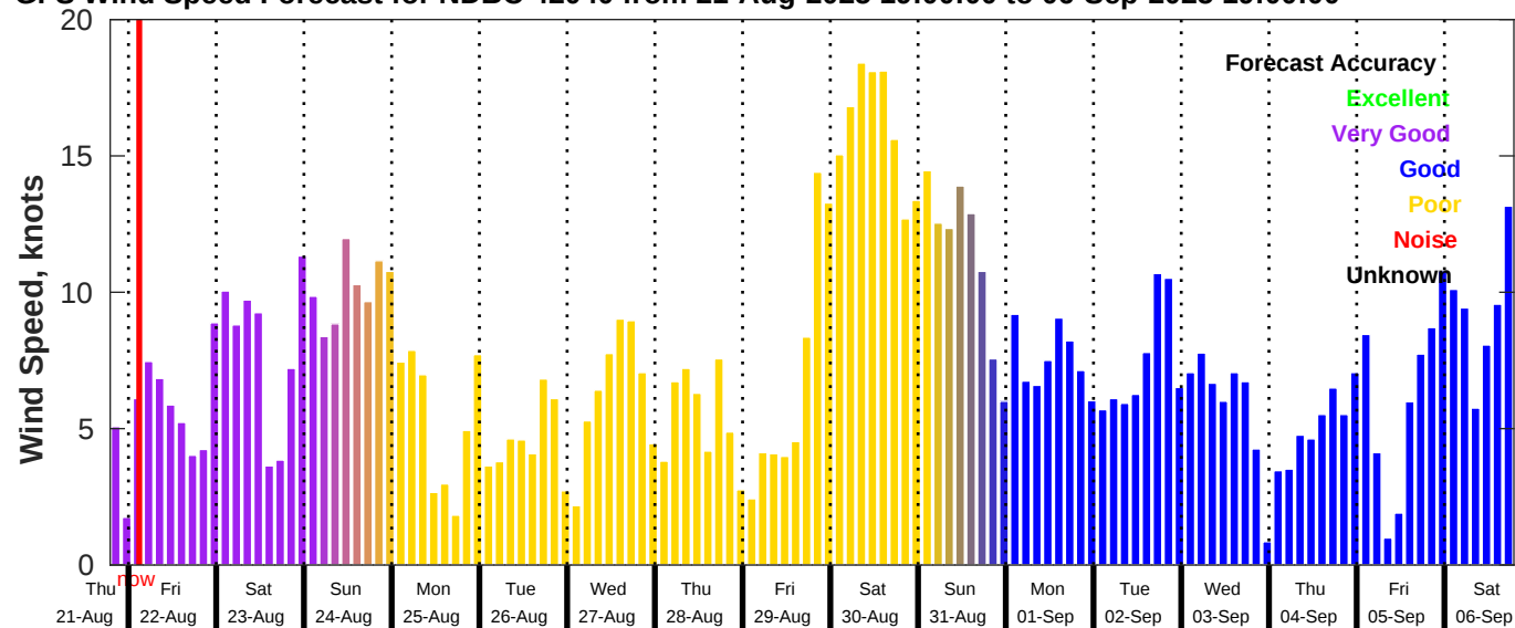
GFS Wind Speed Forecast for NDBC 42040 from 21-Aug-2025 19:00:00 to 06-Sep-2025 19:00:00
