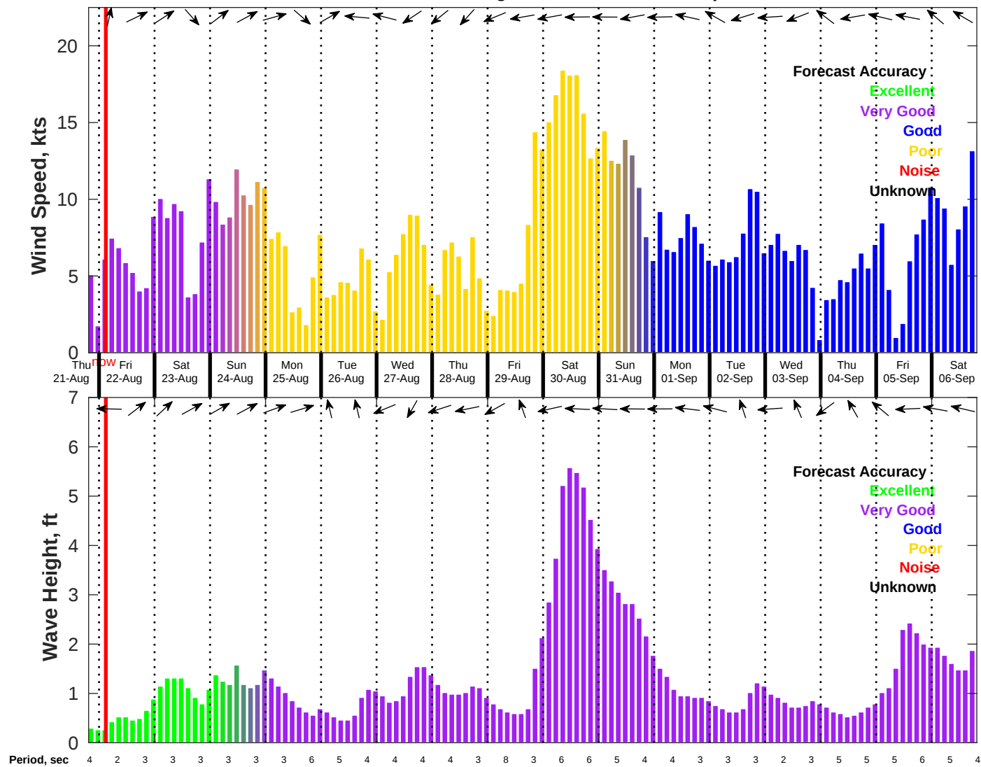
Wind & Wave Forecast for NDBC 42040 from 21-Aug-2025 19:00:00 to 06-Sep-2025 19:00:00
