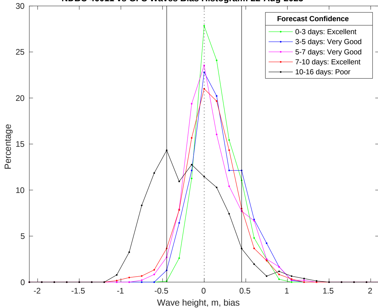
NDBC 46011 vs GFS Waves Bias Histogram: 22-Aug-2025
