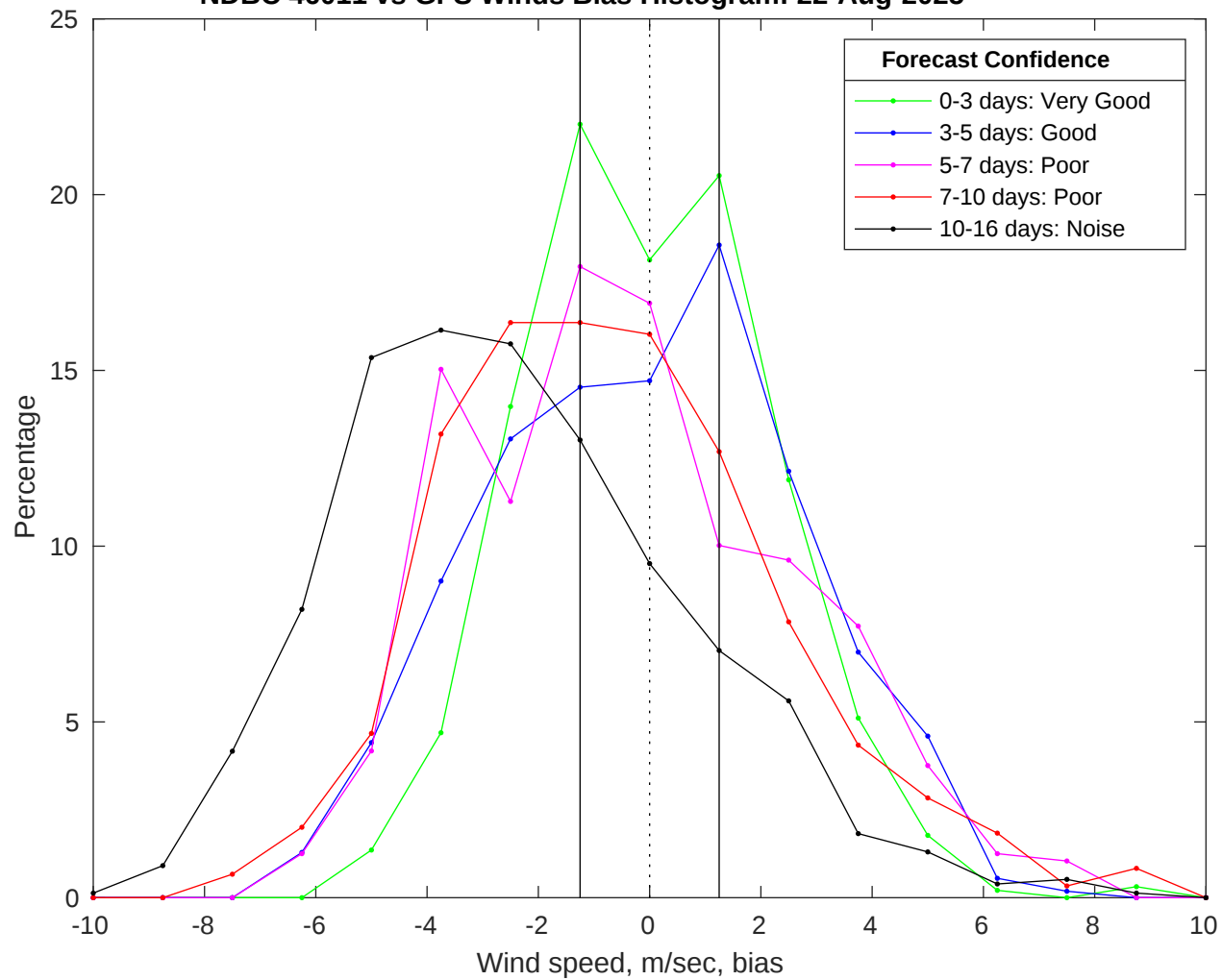
NDBC 46011 vs GFS Winds Bias Histogram: 22-Aug-2025
